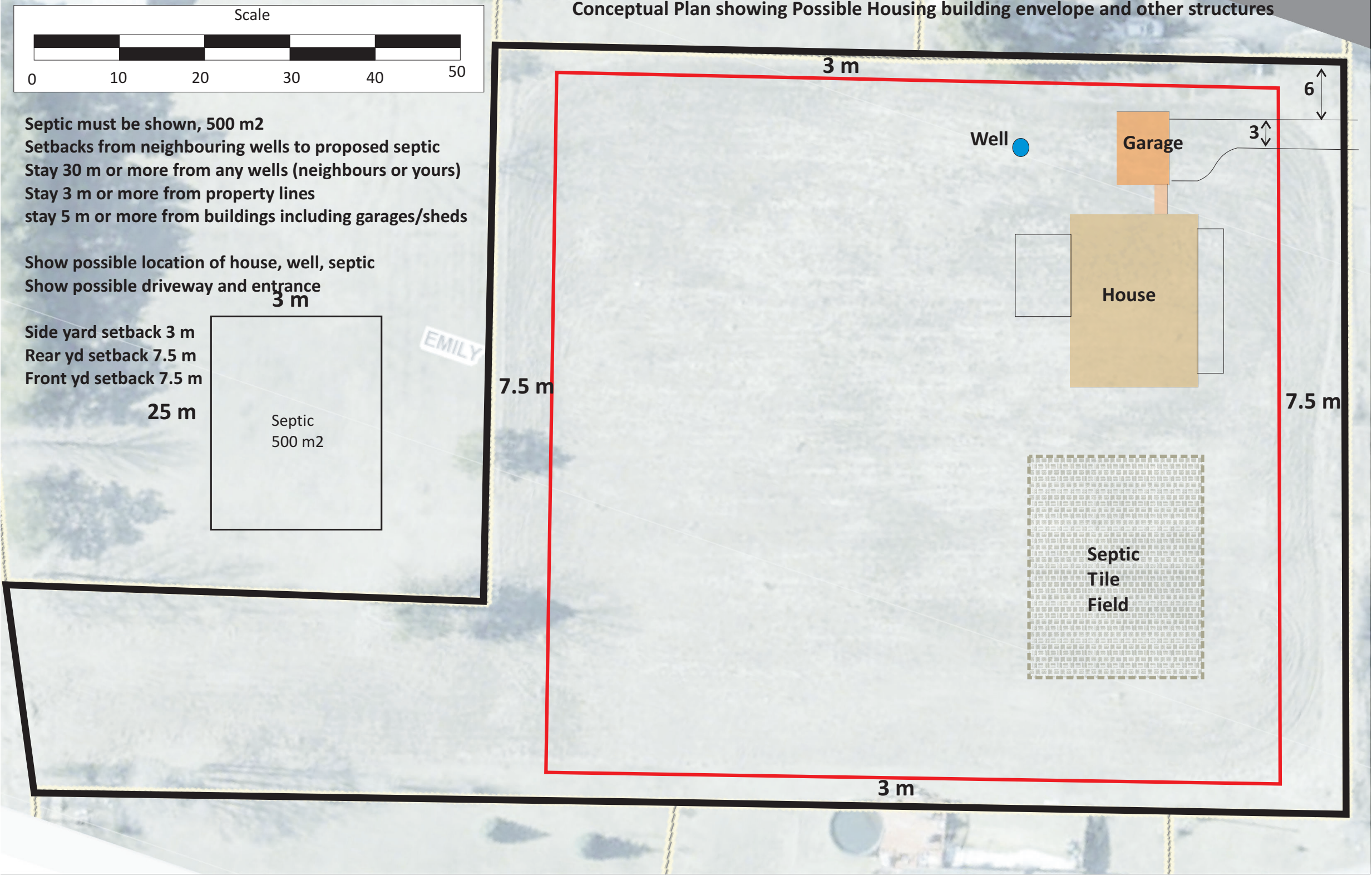
Figure 2 - Conceptual Lot Diagram 614 Shamrock Road, Omemee Part of Lot 13, Concession 7, Geographic Township of Emily City of Kawartha Lakes
